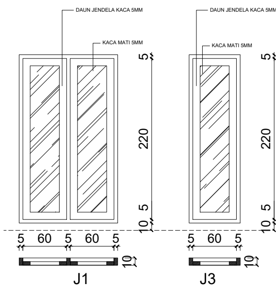
DETAIL KUSEN
